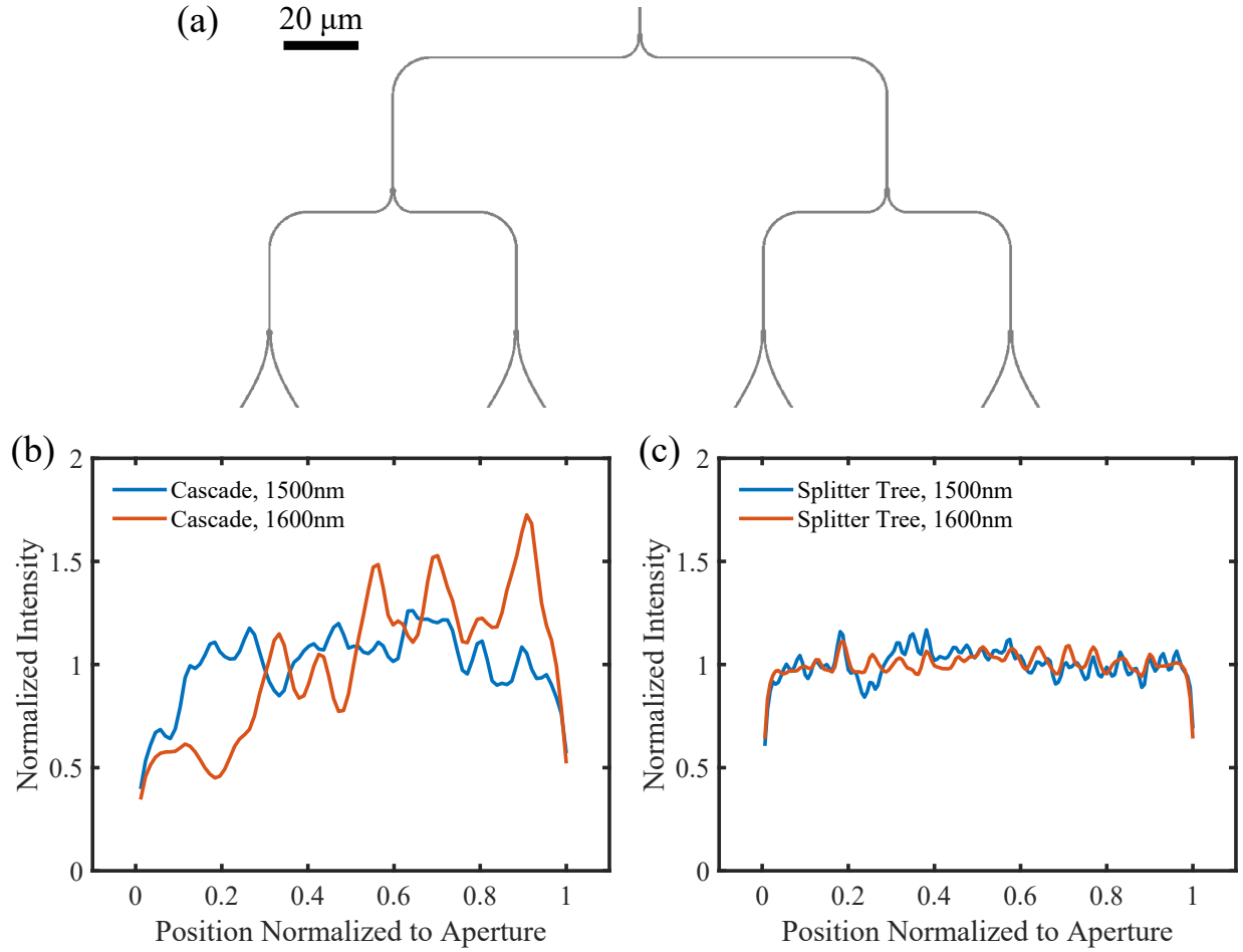
Figure 4.18: (a) The layout of 1 \times 2 splitter-based optical distribution tree available in our process. (b) Measured power distribution across the cascaded directional coupler-based OPA at 1500\text{ nm} and 1600\text{ nm} wavelength. (c) Same data as (b), but from the OPA with the distribution using the design in (a).
